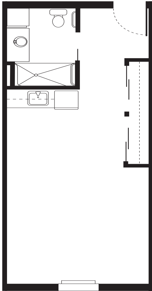
Studio 414 sq. ft.
